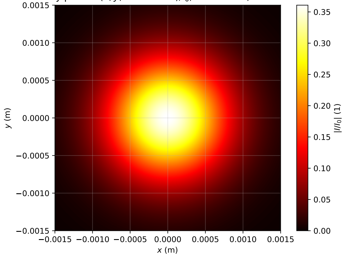
Intensity profile I(x, y, z = 3.742m)/I_0 , P_{in}=0.4P_{cr} , artificial time
